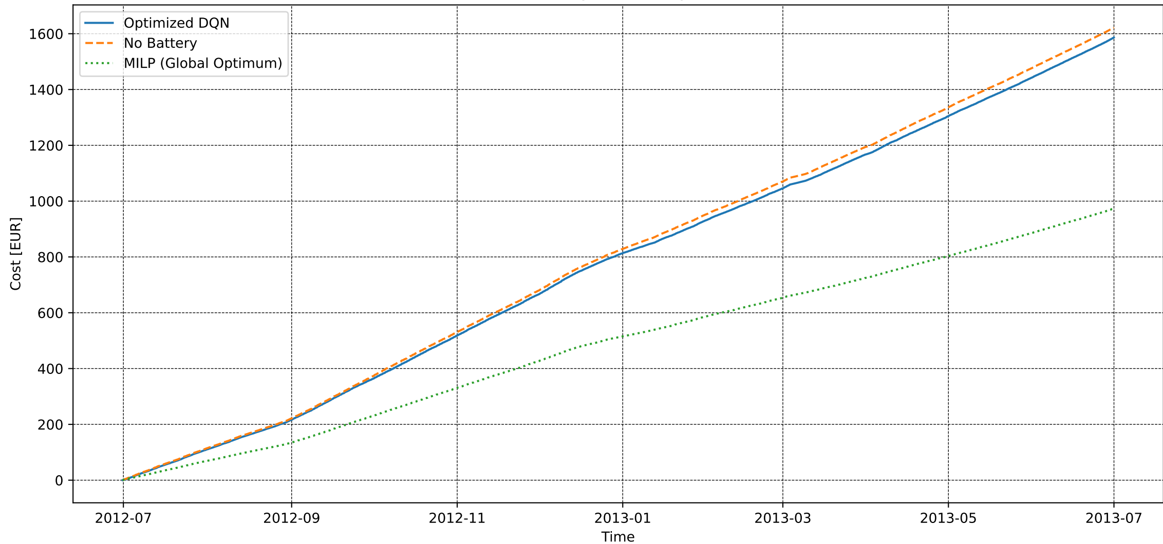
User 158 - Basic Training - Electricity Cost [DQN vs MILP]
